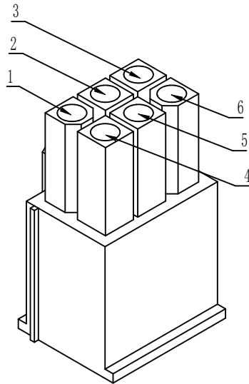
Power Connector:
