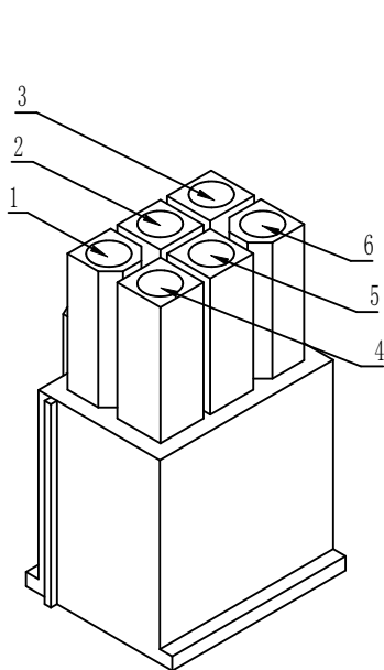
Power Connector: Module-side connector housing: HX41405-6P Module-side connector terminals: HX41406-6R / RT Customer-side connector housing: HX41406-6R Customer-side connector terminals: HX41406-6P / PT
