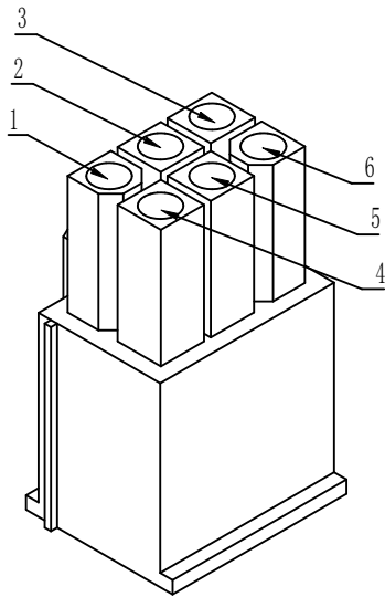
Power Connector: Module-side connector housing: HX41405-6P Module-side connector terminals: HX41406-6R / RT Customer-side connector housing: HX41406-6R Customer-side connector terminals: HX41406-6P / PT
